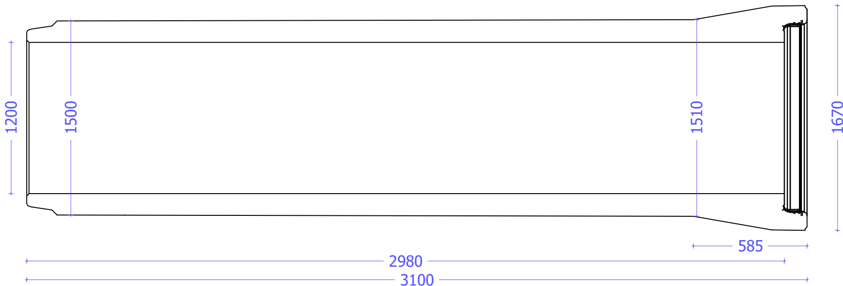
Tuyau standard
