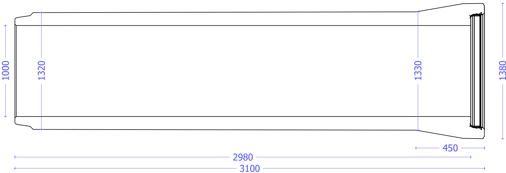
Tuyau standard
